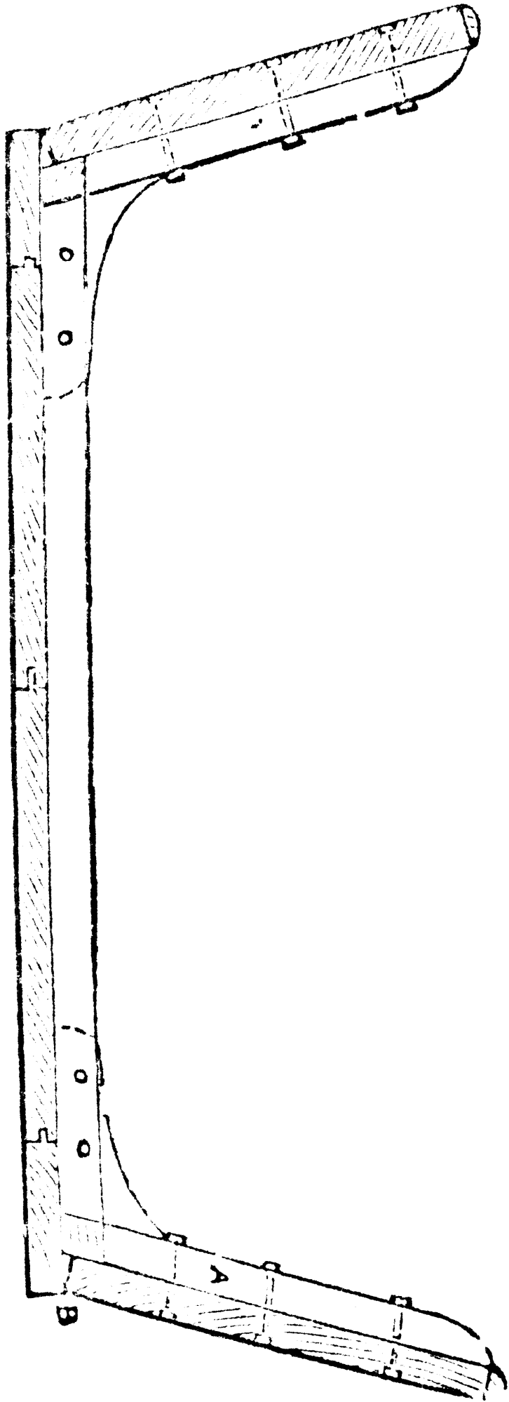
FIG. 15. SECTION OF PUNT SHOWING FRAMES.
